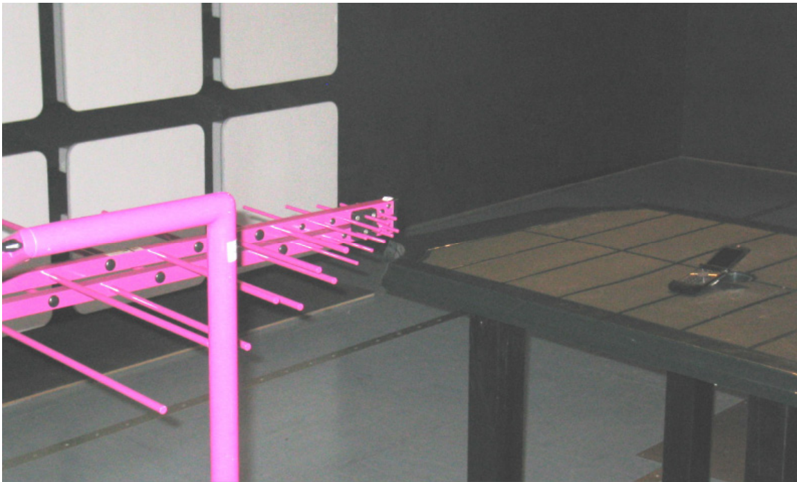
Figure HTD-1: Instrumentation antenna and unit under test in a shielded test chamber (signal generator and transmitting amplifiers are external to chamber)
